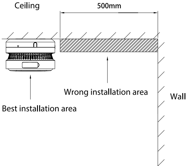
Figure 3-1 Installation position
