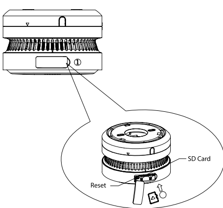
Figure 3-6 SD Card
