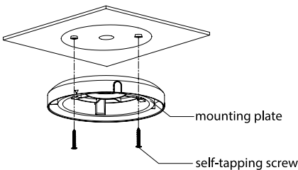
Figure 3-3 Installation (2)
