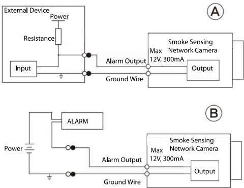
Figure 1-4 Alarm output
