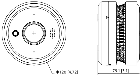
Figure 1-1 Dimensions (mm[inch])
