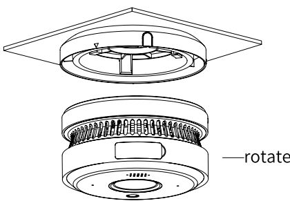
Figure 3-4 Installation (3)
