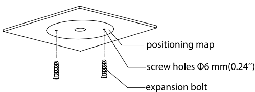
Figure 3-2 Installation (1)
