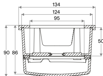
Top View (50 mm Spacer)
