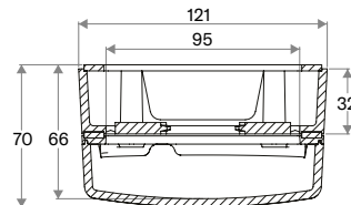
Top View (32 mm Spacer)
