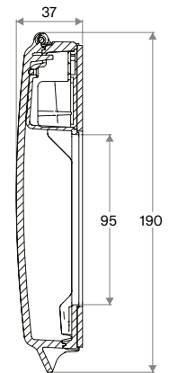
Flush Mount Side View
