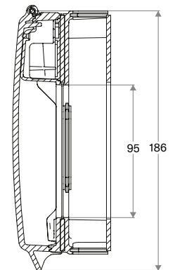
Surface Mount Side View (32 mm Spacer)
