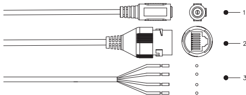
Figure 1-1 Cable list
