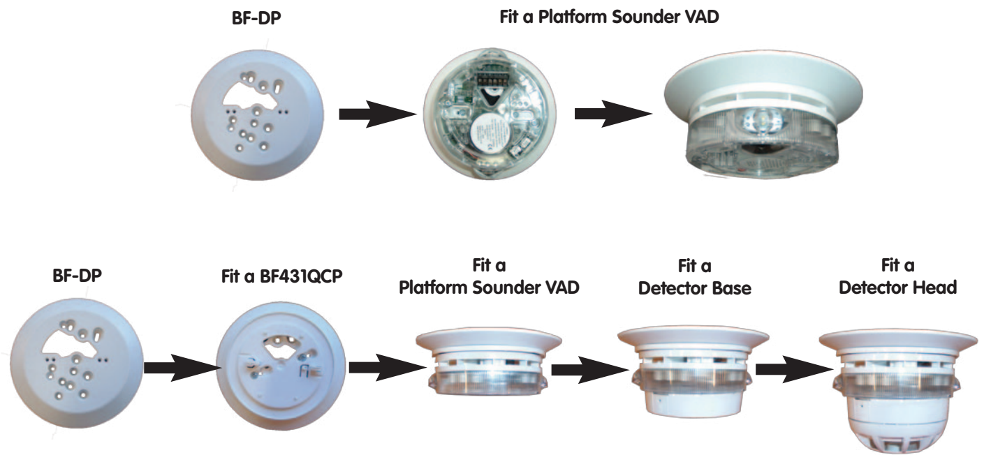
Fig.3 Additional BF-DP Mounting Combinations
